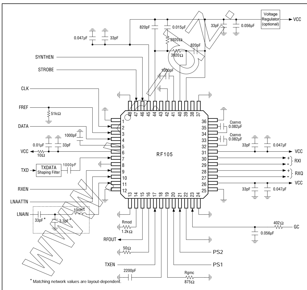
Figure 4. Typical Applications Diagram – RF105
