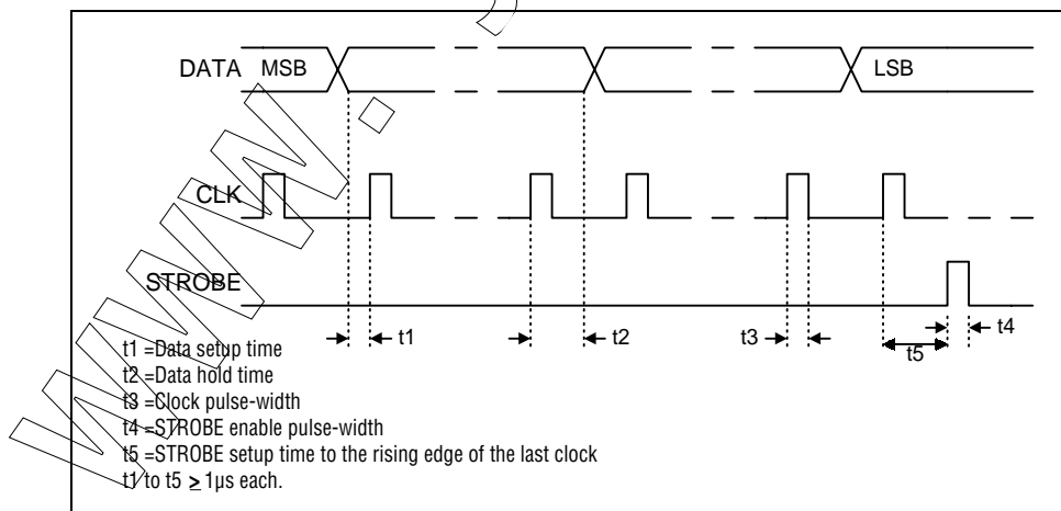
Figure 6. Timing Diagram
