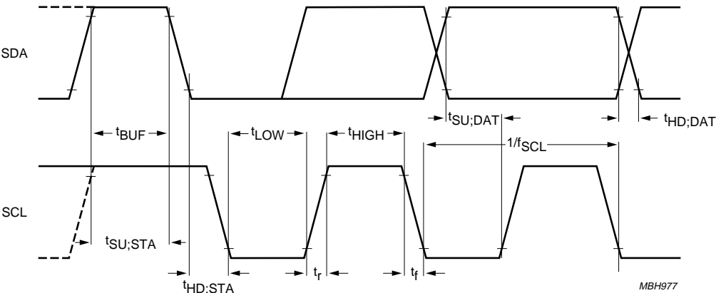
a. Timing diagram 1.
