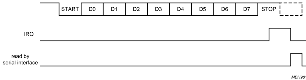
Fig 4. IRQ generation after reading a valid data byte.
