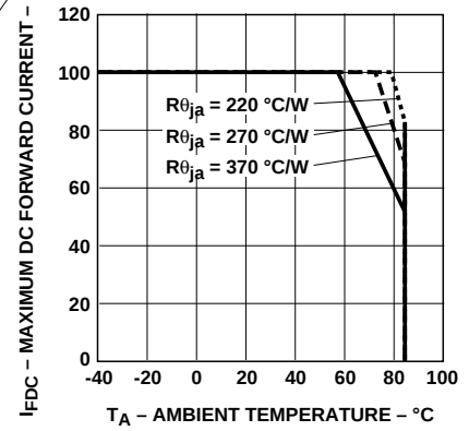
Figure 6. Maximum DC Forward Current vs. Ambient Temperature. Derated Based on T_{JMAX} = 110^{\circ}\text{C} .
