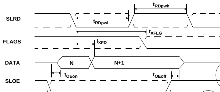
Figure 11-2. Slave FIFO Asynchronous Read Timing Diagram
