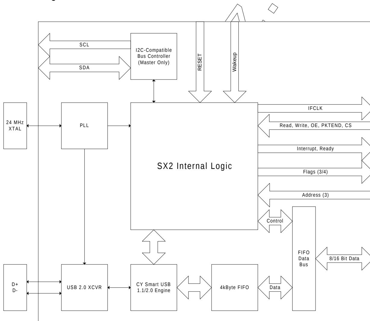
Figure 1-1. Block Diagram
