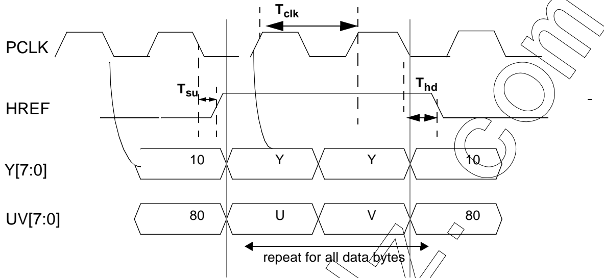
Pixel Data 16-bit Timing (PCLK rising edge latches data bus)
