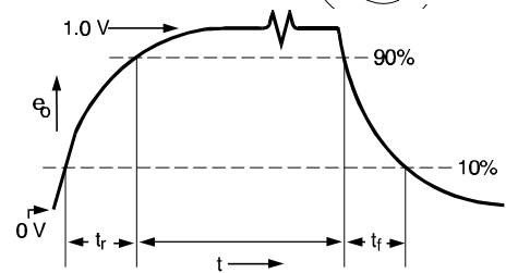
SWITCHING WAVEFORM
