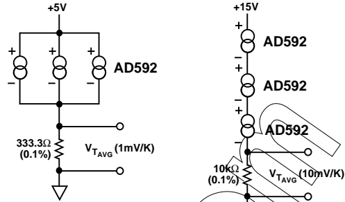
Figure 9. Average and Minimum Temperature Connections
