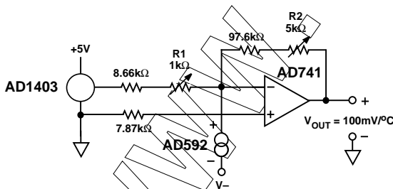
Figure 6. Two Temperature Trim Circuit
