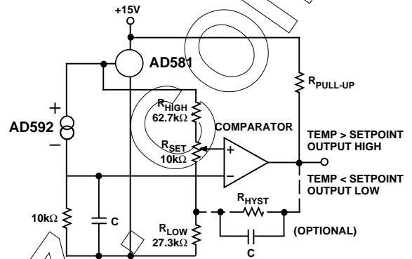
Figure 14. Variable Temperature Thermostat
