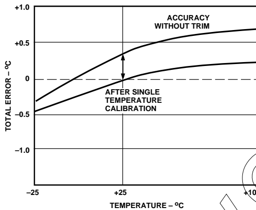
Figure 5. Effect of Scale Factor Trim on Accuracy
