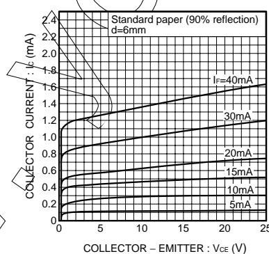
Fig.5 Output characteristics
