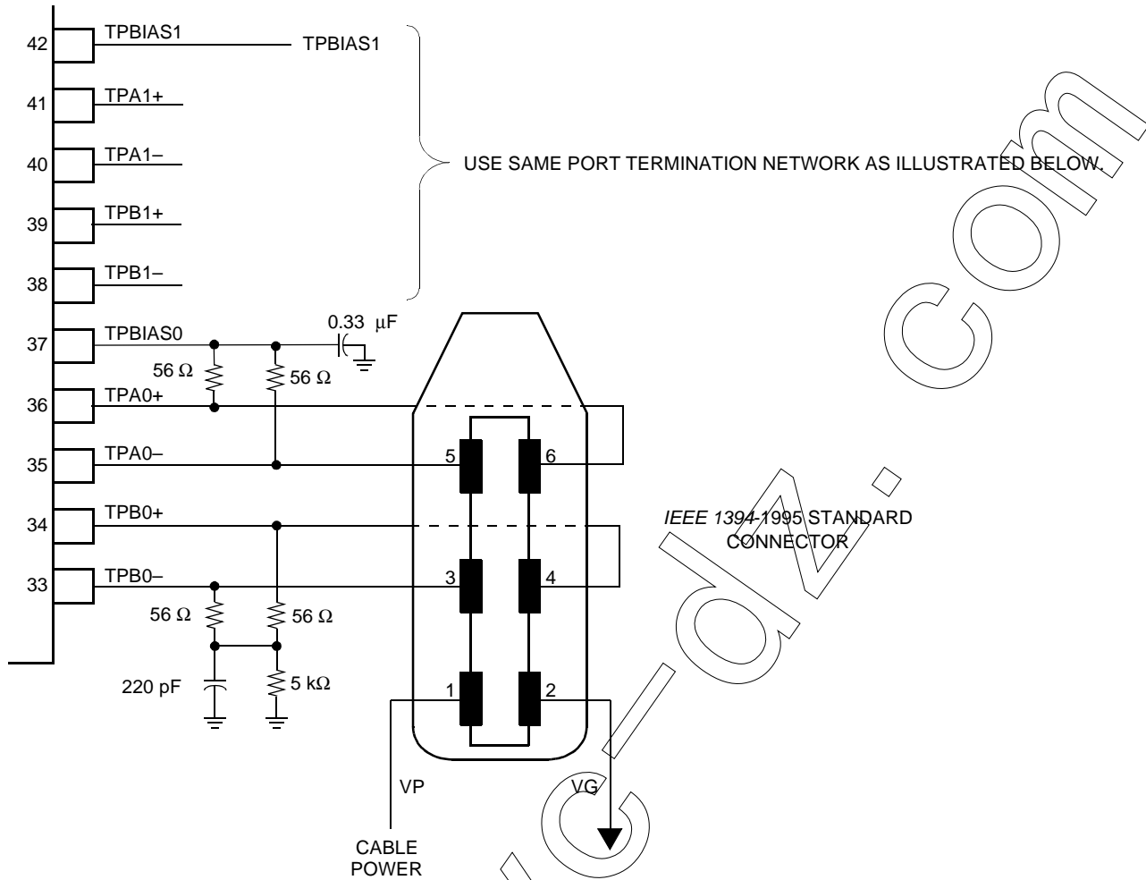
Figure 4. Typical Port Termination Network
