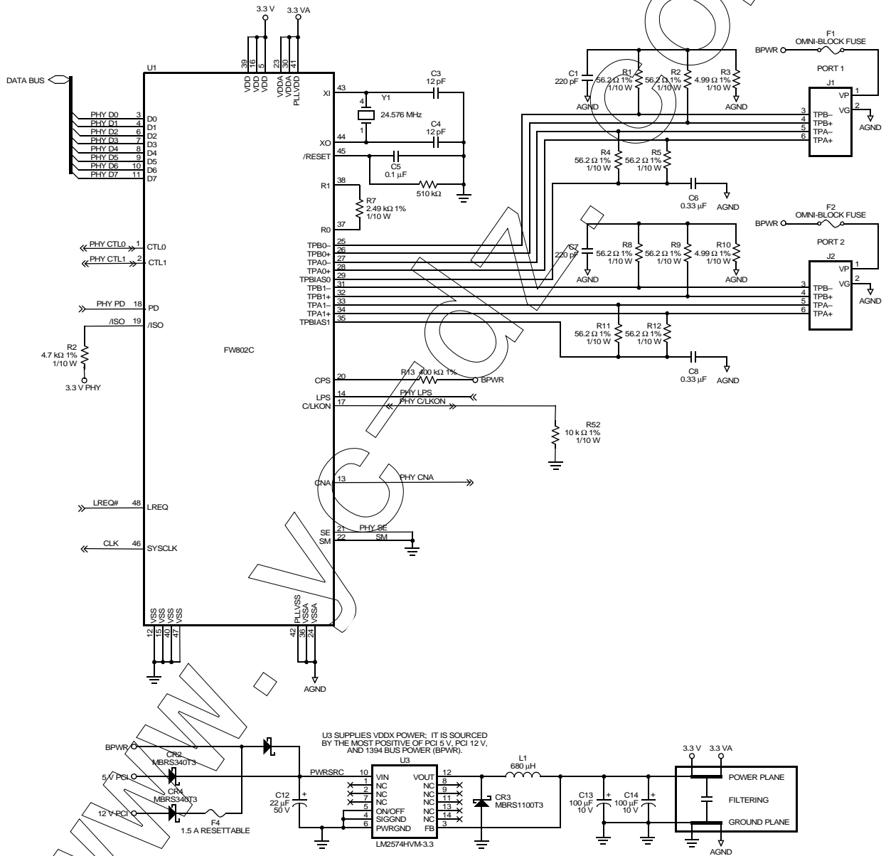
Figure 1. Schematic for the FW802C
