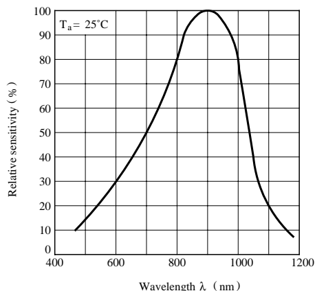
Fig. 9 Spectral Sensitivity
