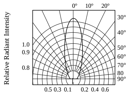
FIG.5 RADIATION DIAGRAM
