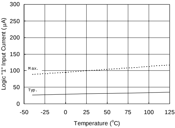
Figure 29C. Logic "1" Input Current vs. Temperature (IR21362 High Side Only)
