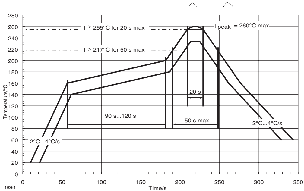
Figure 4. Solder Profile, RSS Recommendation
