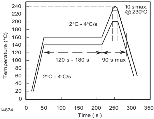
Figure 3. Recommended Solder Profile for Sn/Pb soldering
