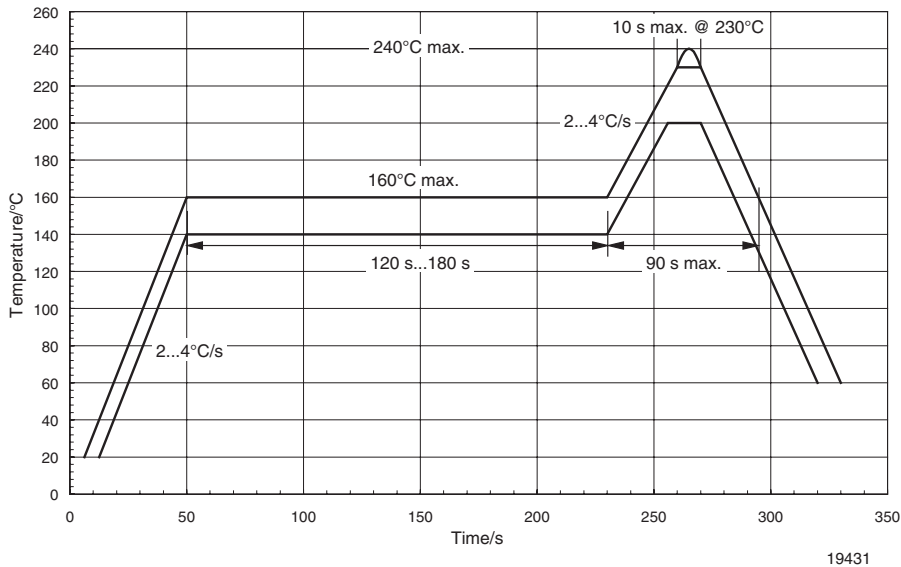
Figure 2. Recommended Solder Profile for Sn/Pb soldering
