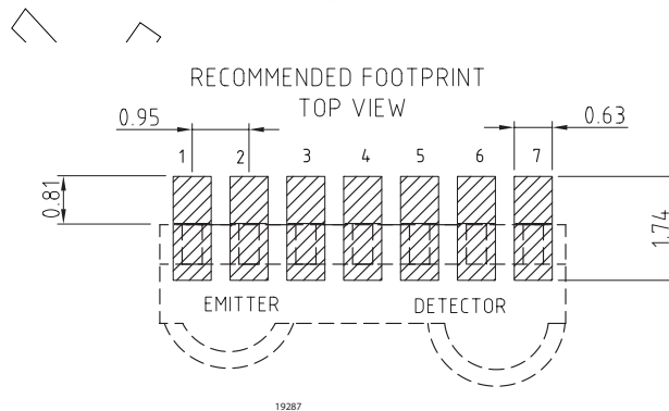
Figure 5: TFBS4652 soldering footprint, tolerance \pm 0.2m , if not otherwise mentioned
