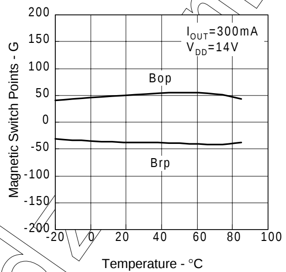
Magnetic Switch Points vs Temperature
