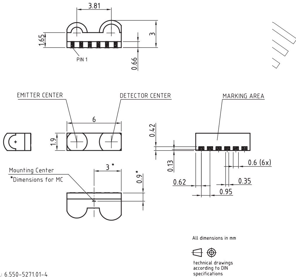
Figure 7. Package drawing
