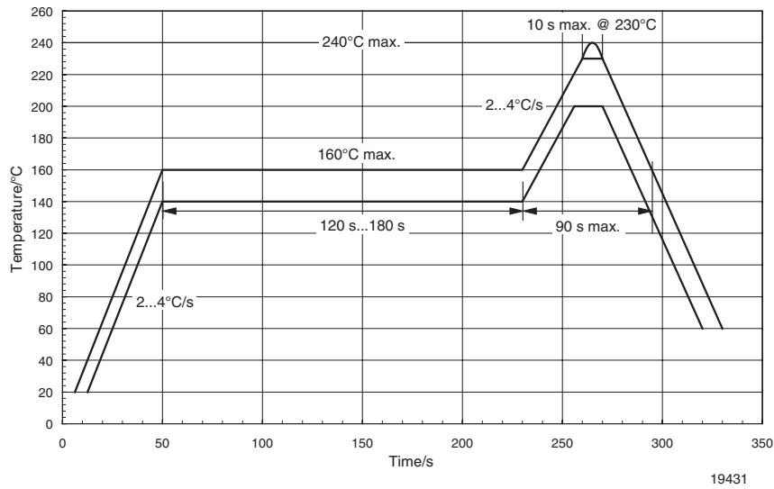
Figure 5. Recommended Solder Profile for Sn/Pb soldering
