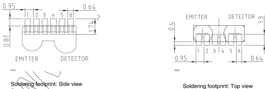
Figure 8. Soldering footprints
