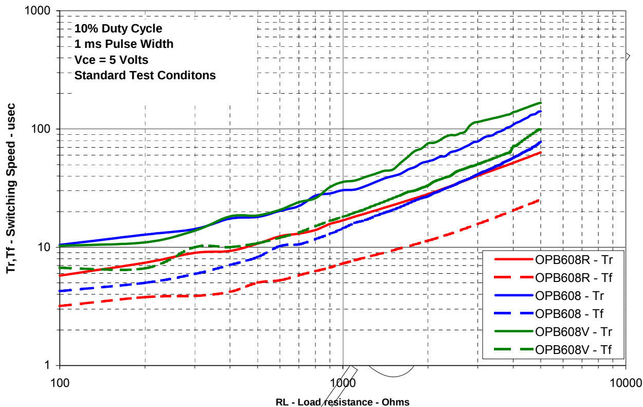
Rise and Fall vs Load Resistance
