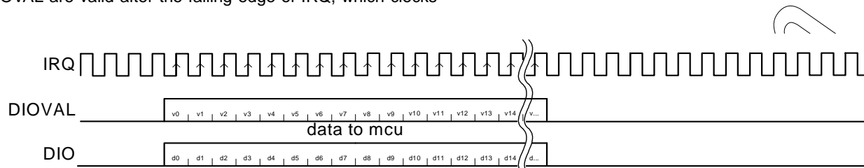
Figure 5-6. DIO Receive Sequence
