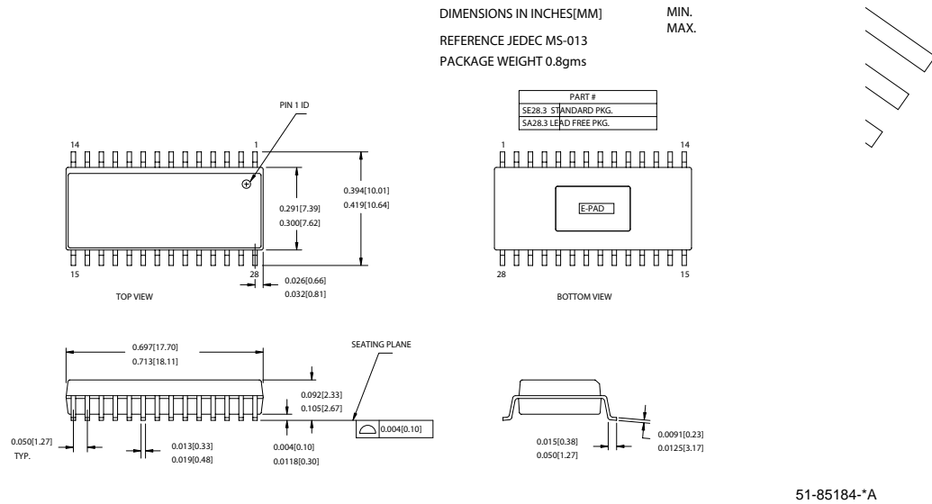
Figure 14-1. 28-pin (300-Mil) SOIC EPAD SE28.3 SOIC
