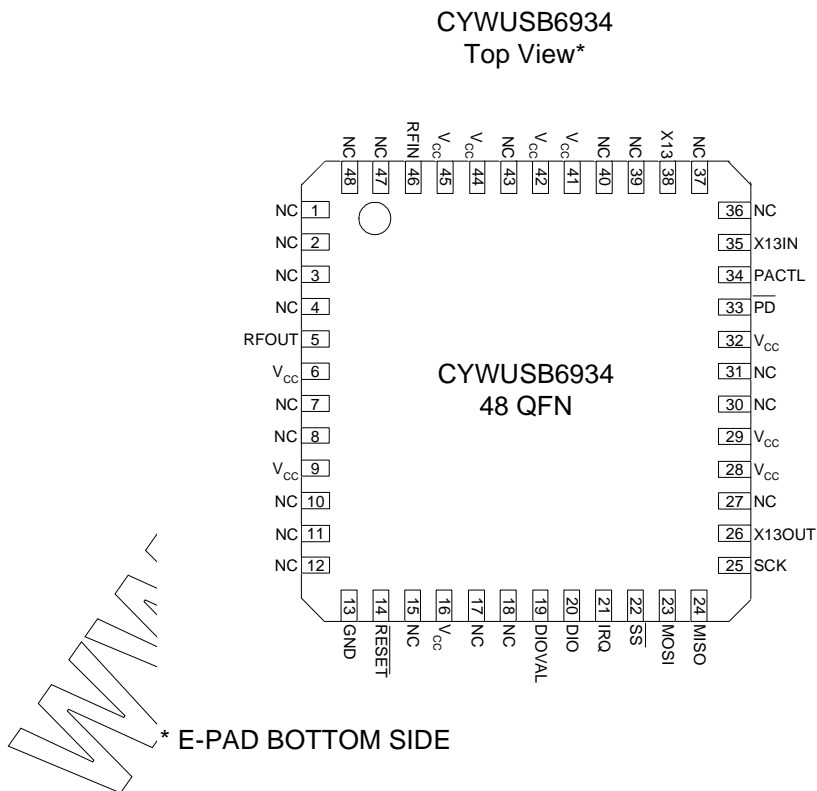
Figure 8-2. CYWUSB6934, 48 QFN – Top View
