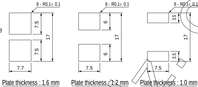
General mounting type
