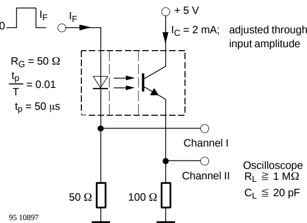
Figure 1. Test circuit, saturated operation
