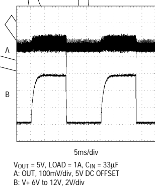
MAX1626 LINE-TRANSIENT RESPONSE
