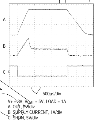
MAX1626 SHUTDOWN RESPONSE TIME AND SUPPLY CURRENT
