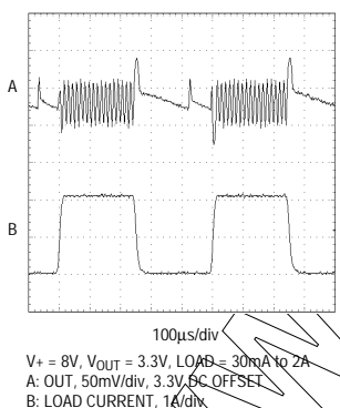
MAX1626 LOAD-TRANSIENT RESPONSE
