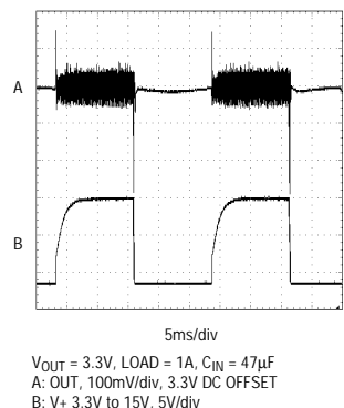
LINE-TRANSIENT RESPONSE FROM 100% DUTY CYCLE
