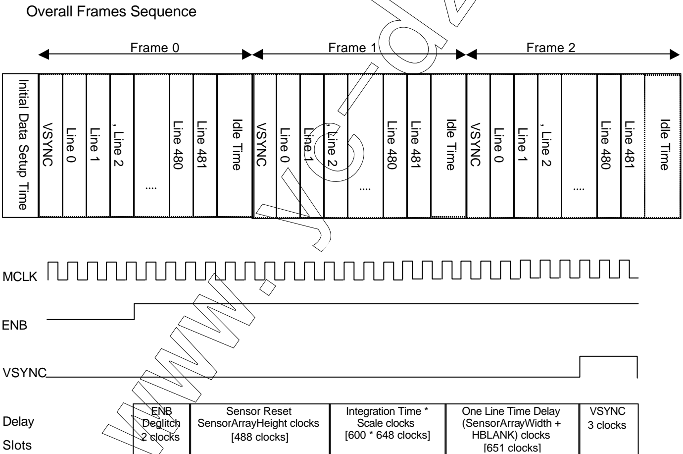
Fig. 5 Initial Data Setup Time after ENB gets active
