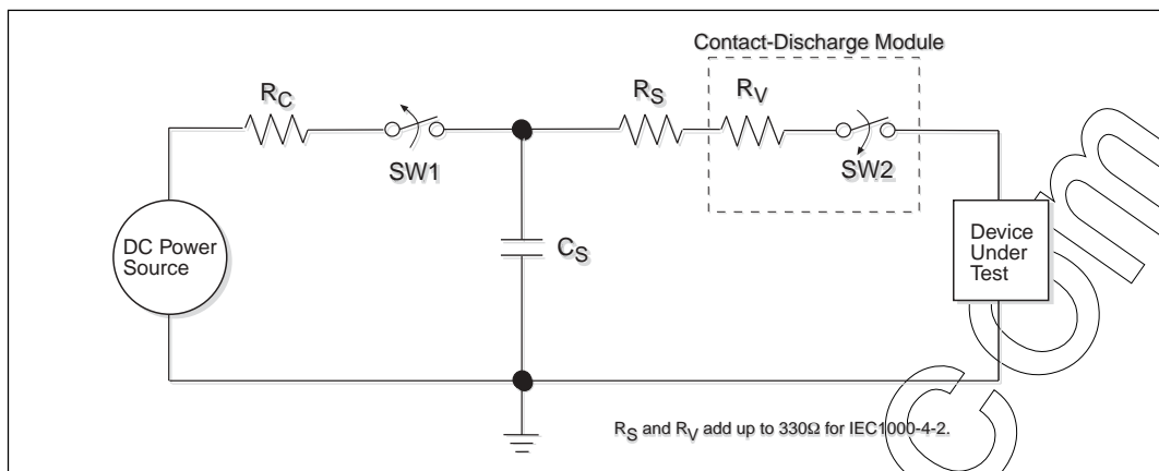
Figure 23. ESD Test Circuit for IEC1000-4-2
