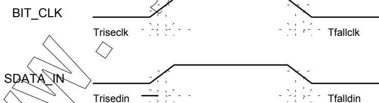
Figure 17. Signal Rise and Fall Times
