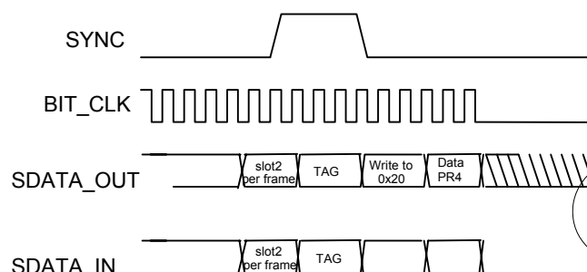
Figure 9. STAC9721/23 Powerdown Timing
