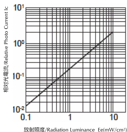
放射照度—相対光電流 特性 Radiation Luminance vs. Relative Photo Current 条件/Condition : T_a = 25^\circ\text{C} , V_{CE} = 5\text{V}
