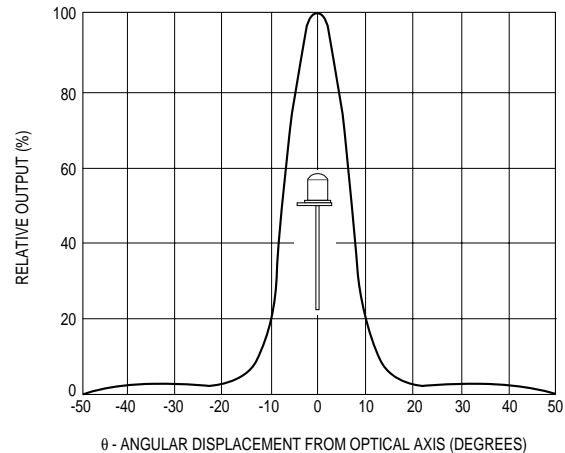
Figure 5. Typical Radiation Pattern
