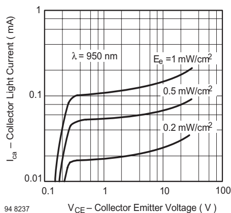
Fig. 5 Collector Light Current vs. Collector Emitter Voltage
