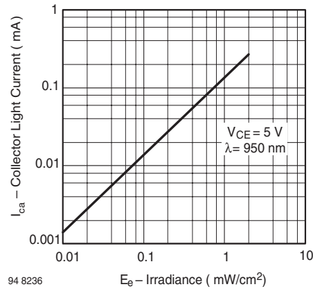
Fig. 4 Collector Light Current vs. Irradiance
