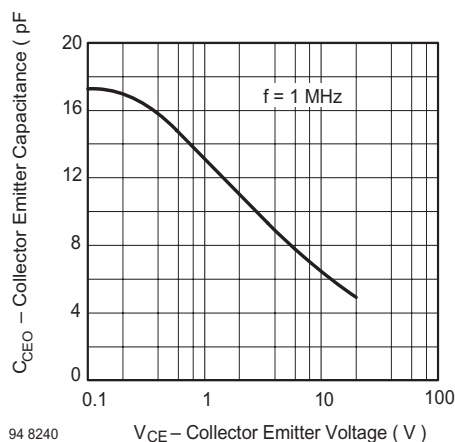
Fig. 6 Collector Emitter Capacitance vs. Collector Emitter Voltage
