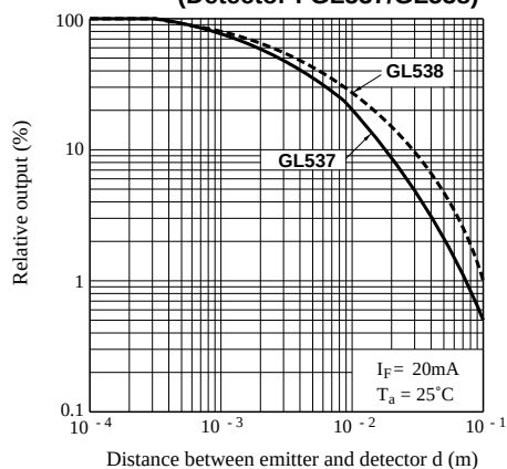
Fig. 9 Relative Output vs. Distance (Detector : GL537/GL538)
