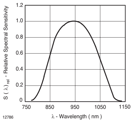
Fig. 5 Relative Spectral Sensitivity vs. Wavelength
