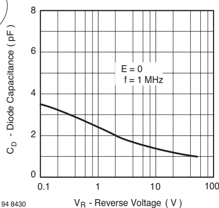
Fig. 4 Diode Capacitance vs. Reverse Voltage
