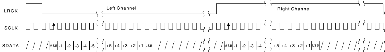
Figure 2. I²S Data
