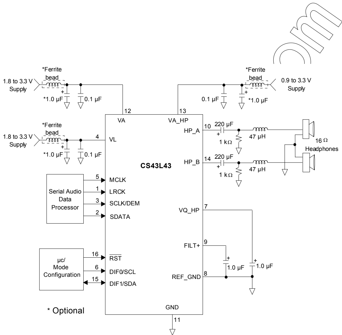
Figure 1. Typical Connection Diagram
