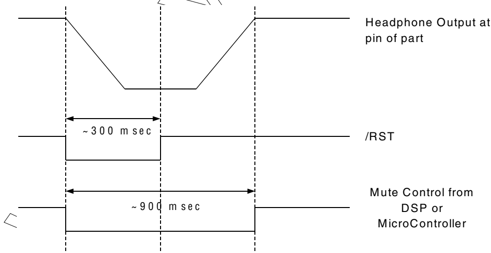
Figure 7. Timing for Headphone Mute
