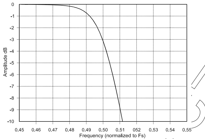
Figure 13. Single-Speed Transition Band (Detail)
