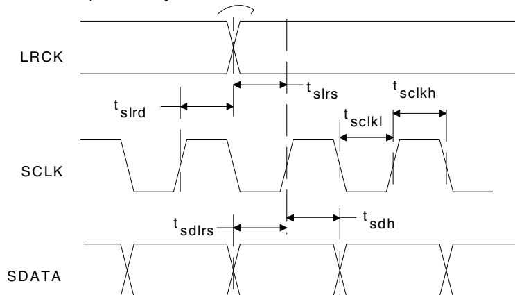
Figure 19. External Serial Mode Input Timing
