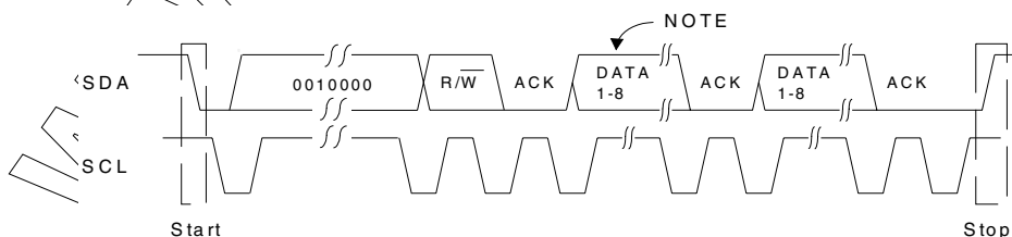
Figure 8. Control Port Timing
