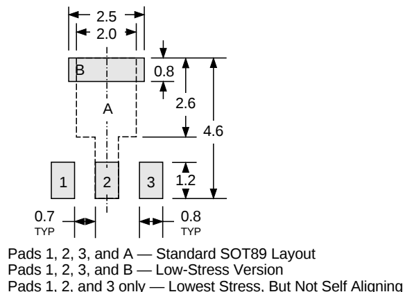
Dwg. MA-012-3 mm
