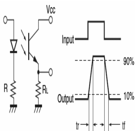
応答速度測定回路 Response Time Measuring Circuit
