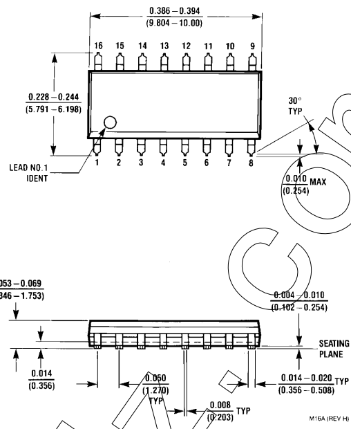
16-Lead Small Outline Molded Package (M) Order Number DM74LS161AM or DM74LS163AM NS Package Number M16A
