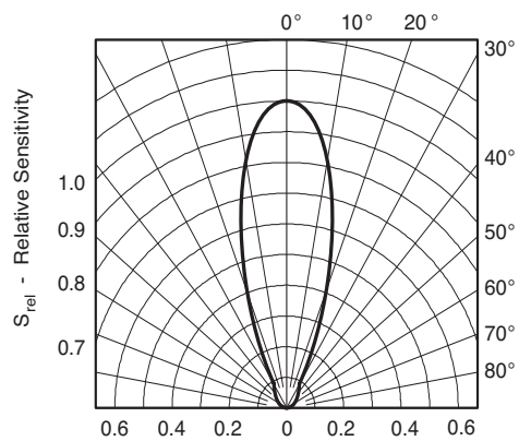
Fig. 5 Relative Radiant Sensitivity vs. Angular Displacement
