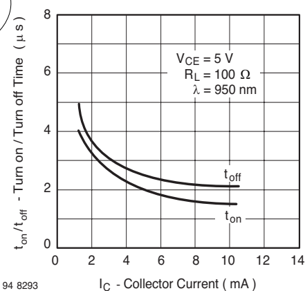
Fig. 4 Turn On/Turn Off Time vs. Collector Current
