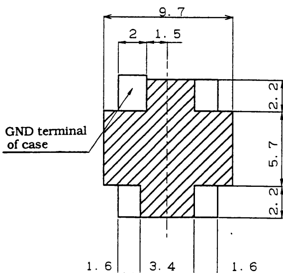
Example of pattern looking from PCB (Reference)
