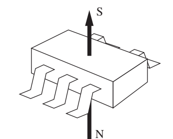
Direction of applied magnetic field
