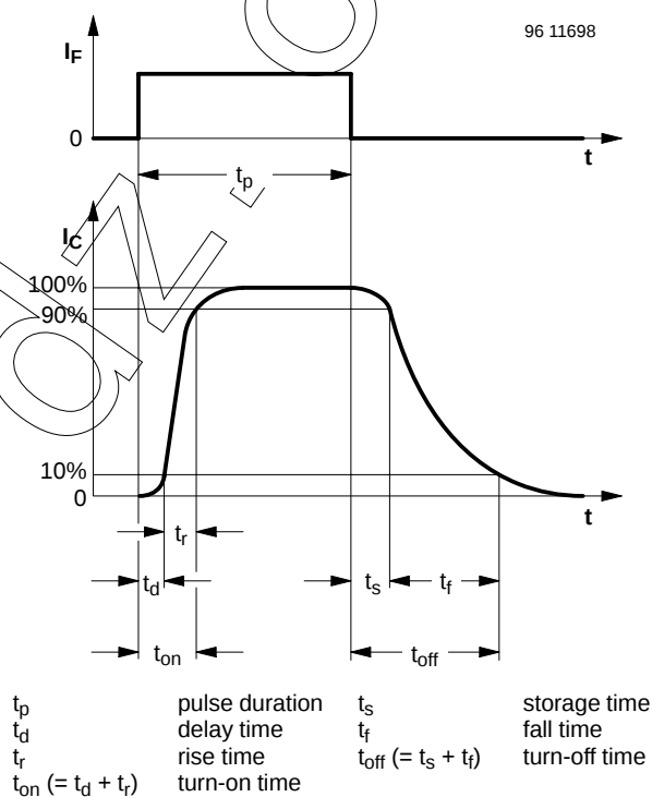
Figure 2. Switching times
