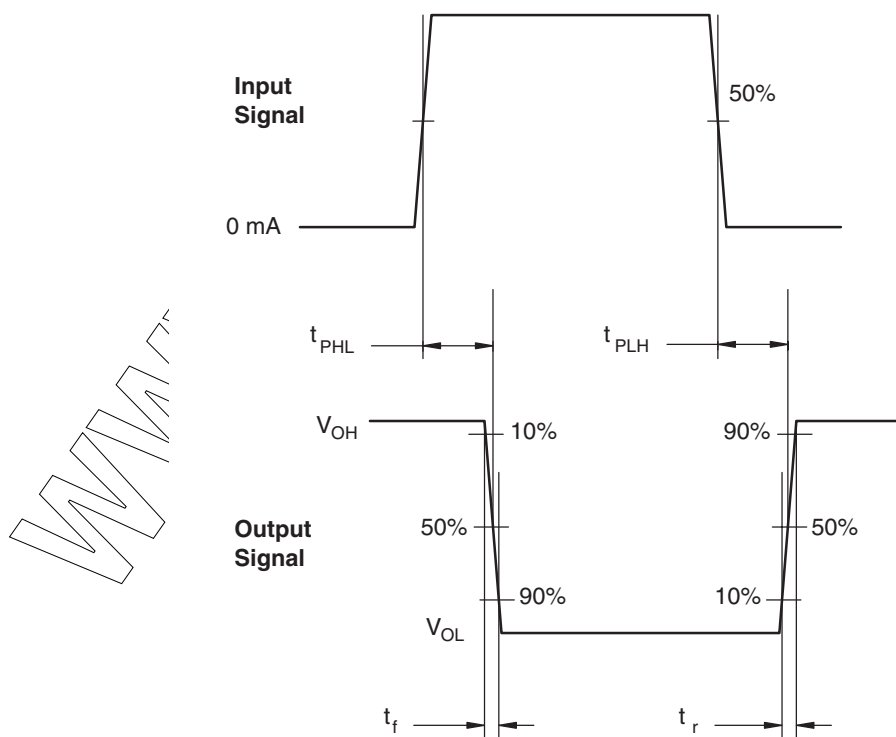
Fig. 8 Switching Test Curve for Inverters
