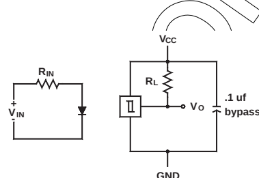
Figure 10. Typical Operating Circuit
