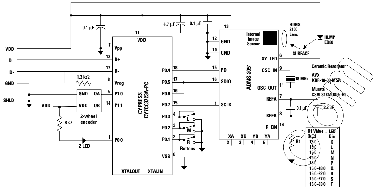
Figure 3. Circuit-level block diagram for optical mouse solution using ADNS-2051 optical mouse sensor.
