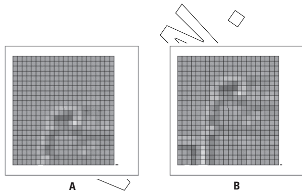
Figure 1. The Navigation Engine identifies common features in sequential images to determine the direction and amount of mouse movement. Image B was taken while the mouse was moving, a short time after image A.
