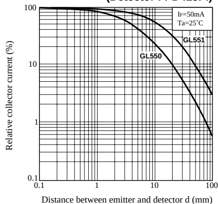
Fig. 9 Relative Collector Current vs. Distance (Detector : PD413PI)
