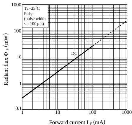
Fig. 8 Radiant Flux vs. Forward Current
