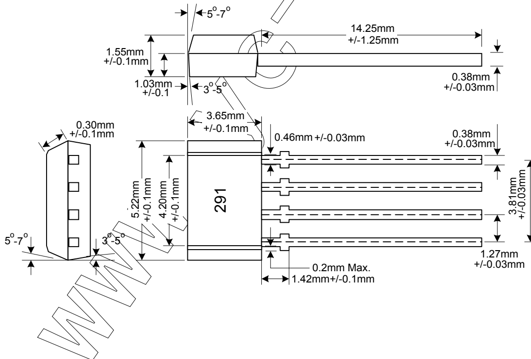
Package Dimension
