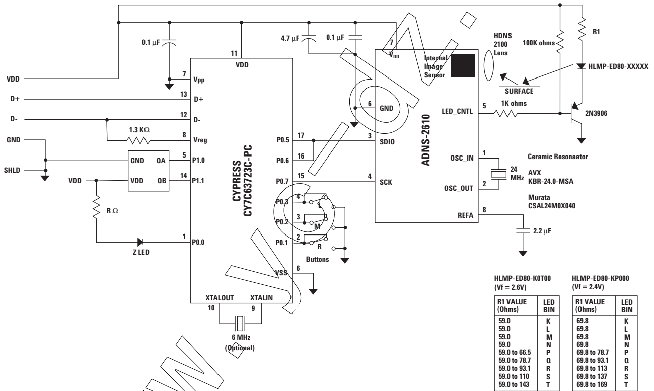
Figure 3. Circuit-level block diagram for optical mouse solution using an Agilent ADNS-2610 optical mouse sensor.
