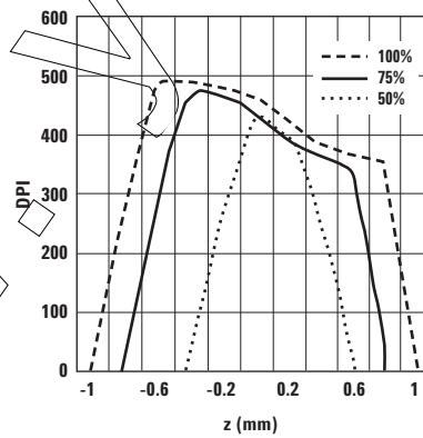
Figure 19. Typical Resolution vs. Height at different LED current levels on black copy.
