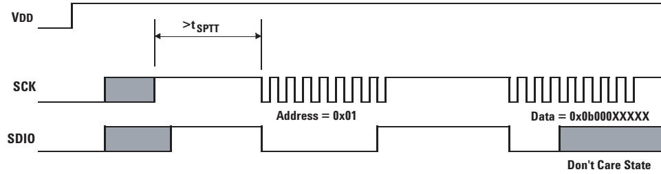
Figure 30. Power-up serial port timer sequence.
