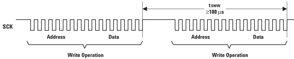
Figure 26. Timing between two write commands.
