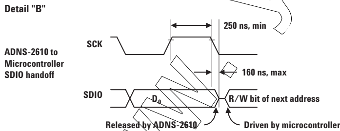
Figure 24. ADNS-2610 to microcontroller SDIO handoff.
