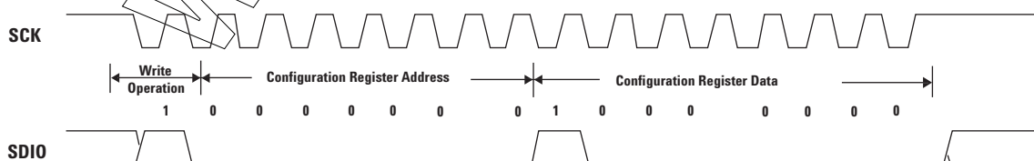
Figure 32. Soft reset configuration register writing operation.
