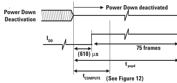
Figure 11. Power up timing mode.
