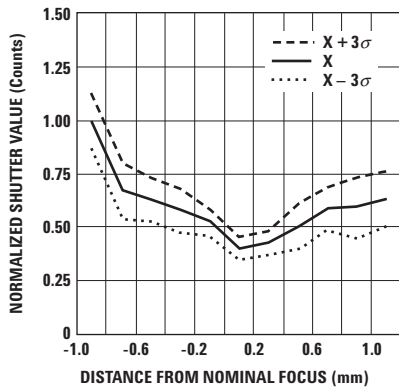
Figure 34. Typical Mean Shutter vs. z (white paper).
