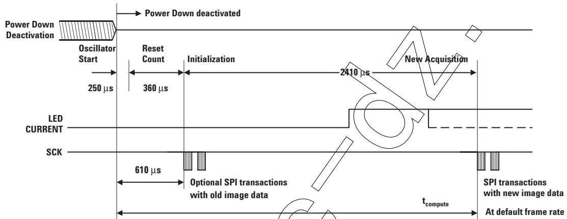
Figure 12. Details of wake-up timing after PD.
