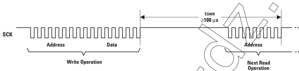
Figure 27. Timing between write and read commands.
