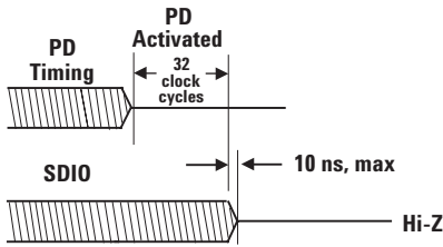
Figure 25. SDIO Hi-z state and timing.
