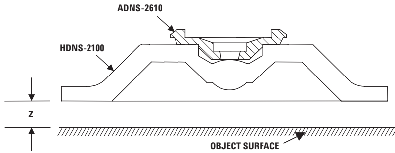
Figure 10. Distance from lens reference plane to surface.
