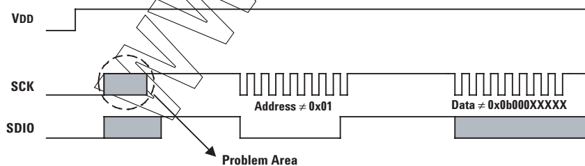
Figure 29. Power-up serial port sequence.
