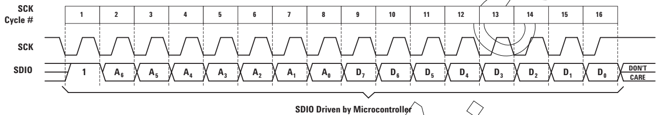
Figure 20. Write operation.
