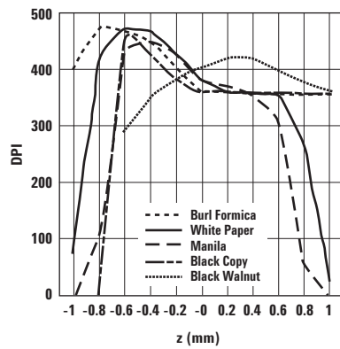
Figure 15. Typical Resolution vs. Z (comparative surfaces)
