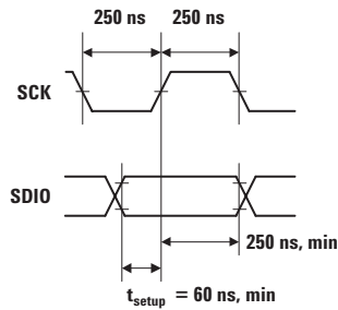
Figure 21. SDIO setup and hold times SCK pulse width.
