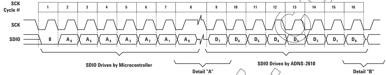
Figure 22. Read operation.
