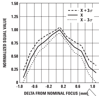
Figure 33. Typical Mean SQUAL vs. z (white paper).
