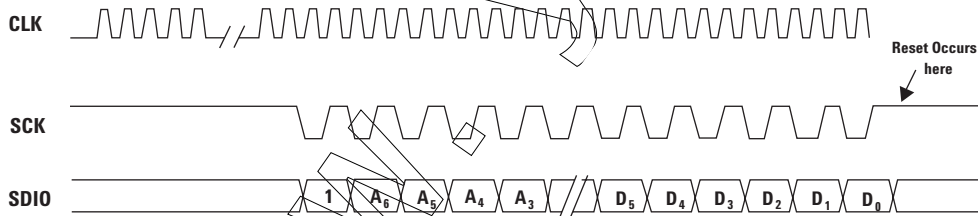
Figure 31. ADNS-2610 soft reset sequence timing.
