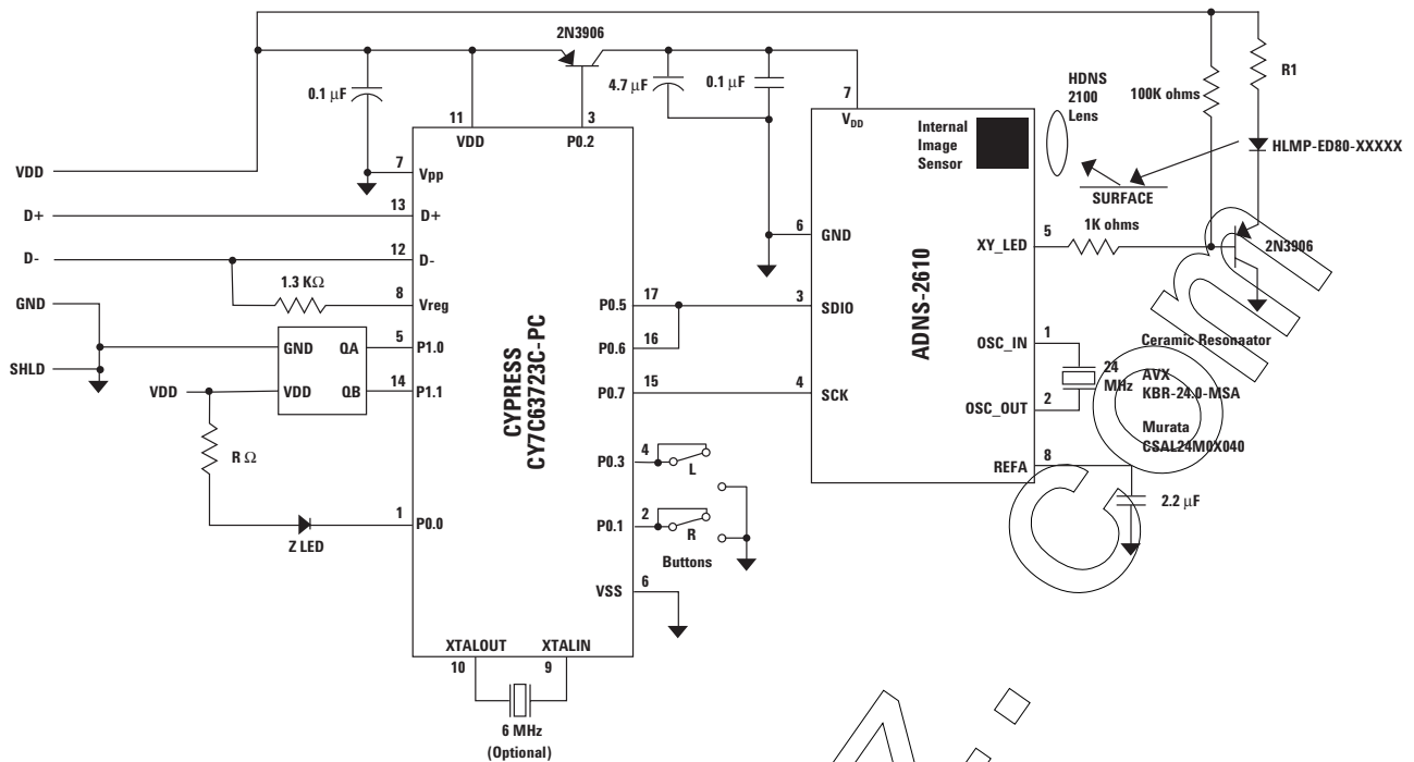
Figure 9. Circuit block diagram with reset circuit for a typical corded optical mouse using an Agilent ADNS-2610 optical mouse sensor.
