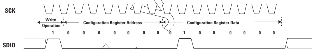
Figure 14. Power-down configuration register writing operation.
