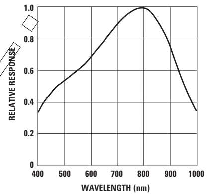
Figure 17. Wavelength Responsivity [1] .
