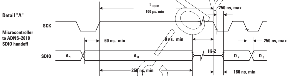
Figure 23. Microcontroller to ADNS-2610 SDIO handoff.
