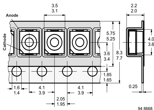
Figure 12. Tape Dimensions in mm for PLCC-2
