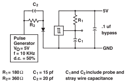
Switching Speed Test Circuit
