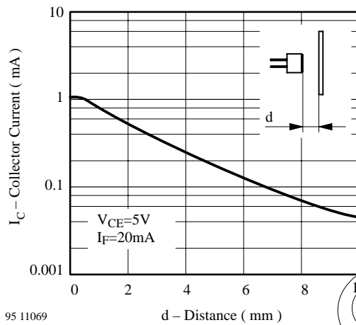
Figure 9. Collector Current vs. Distance
