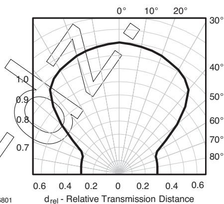
Figure 11. Directivity
